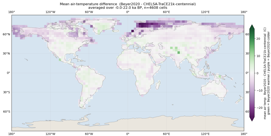
Figure 8. Mean air-temperature difference, Beyer2020 – CHLSA-TraCE21k-centennial (0–22 ka), sampled at the TraCE-21k grid and averaged over the pair’s shared time window (green = first archive warmer, purple = colder).
