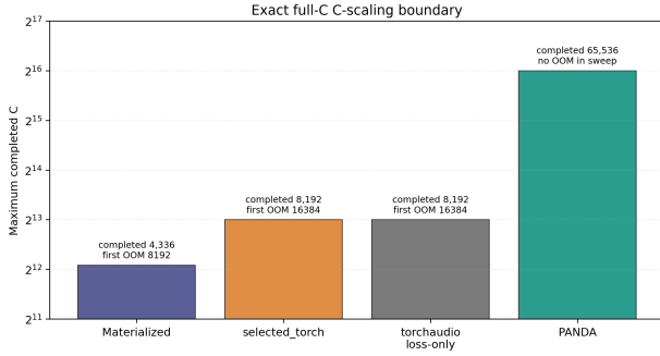
Figure 4. Exact full- C C-scaling boundary. Materialized full logits first OOM at C = 8192 ; guarded k2_mi/PANDA completes through C = 65536 . Scope is integrated_path for materialized, selected_torch, and guarded k2_mi/PANDA rows, and loss_only for the torchaudio row. The corresponding PyTorch peak allocated/reserved MiB values are reported in Table 2. Synthetic- C rows support the C1 mechanism claim.
