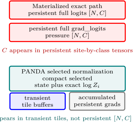
Figure 3. Persistent memory term removed by PANDA. The materialized exact path stores persistent full [N, C] logits and exposes full grad_logits pressure at fixed sites. PANDA keeps compact selected emissions and log Z_i state, while full- C quantities are recomputed in tile-local transient buffers. This conceptual diagram explains the memory/OOM mechanism; measured PyTorch peak allocated/reserved MiB values are reported in the evaluation tables.
