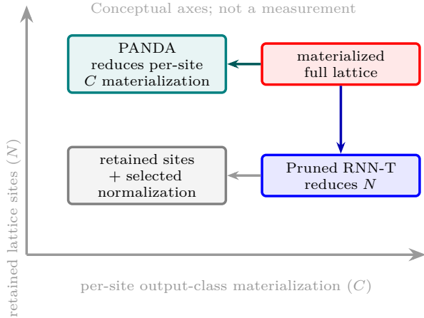
Figure 6. Why pruning and selected normalization compose. Pruned RNN-T reduces the number of retained lattice sites N , while PANDA removes persistent per-site full- C materialization. This is a conceptual axes diagram rather than a measured row; the measured retained-site rows in Table 4 use integrated_path scope and report PyTorch peak allocated/reserved MiB.
