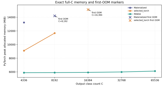
Figure 5. PyTorch peak allocated memory for the exact full- C fixed full-mode sweep. Scope is integrated_path for the plotted materialized, selected_torch, and guarded k2_mi/PANDA rows. The y-axis is PyTorch peak allocated memory in MiB; reserved MiB and row scopes are reported in Table 2. Cross markers denote first-OOM failure attempts. Synthetic- C rows support the C1 mechanism claim.
