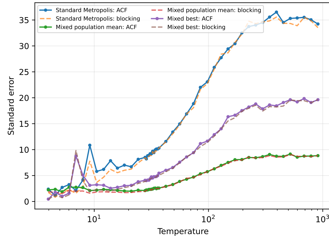
Uncertainty of the mean
