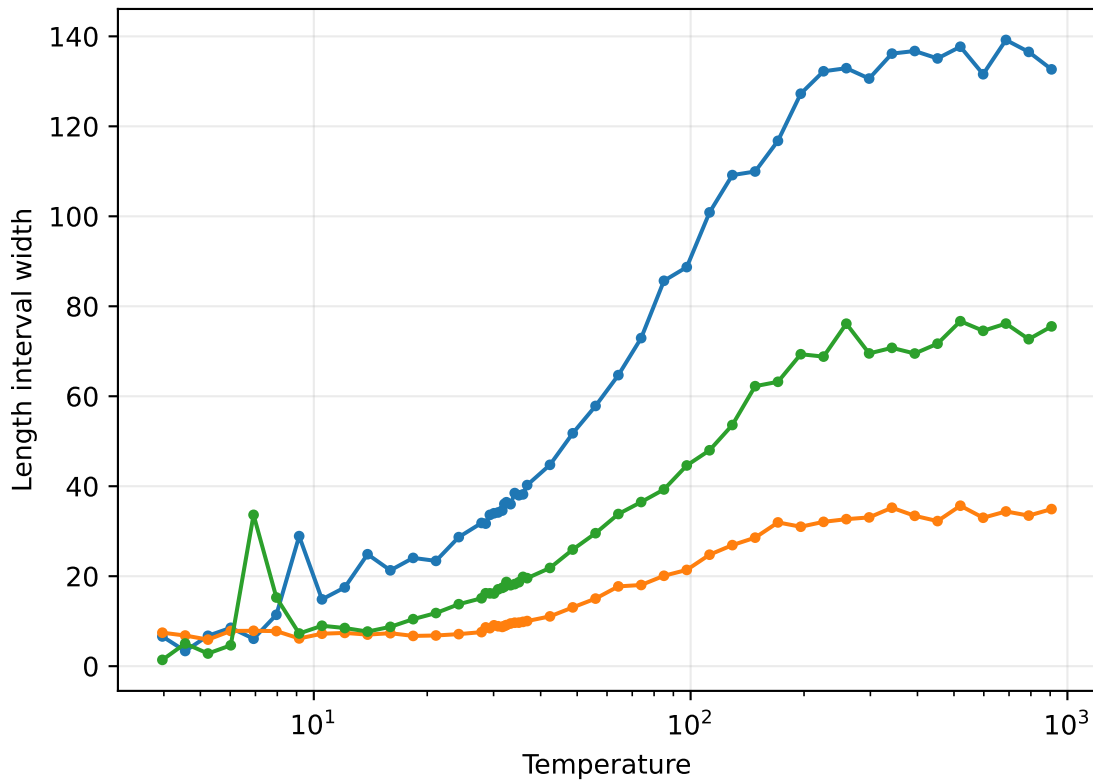
Bootstrap 95% interval width
