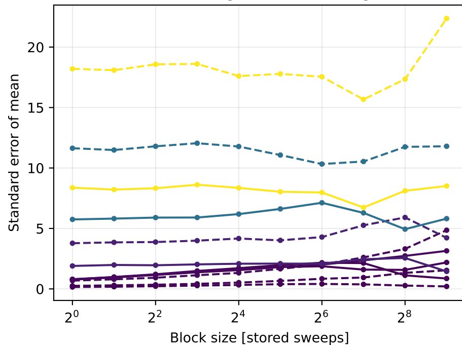
Mixed diagnostics: blocking
