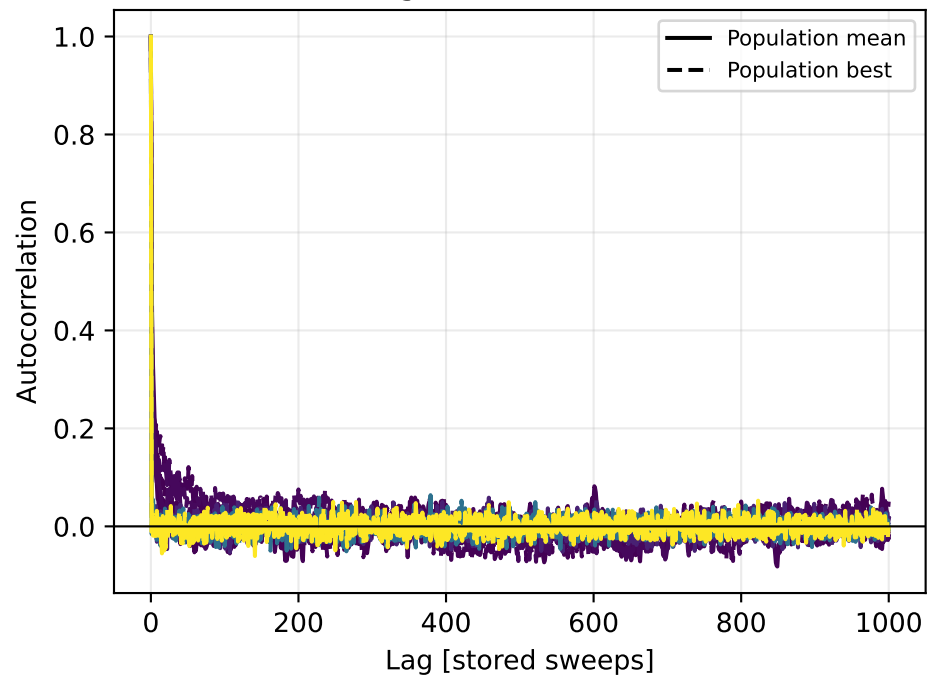
Mixed diagnostics: autocorrelation
