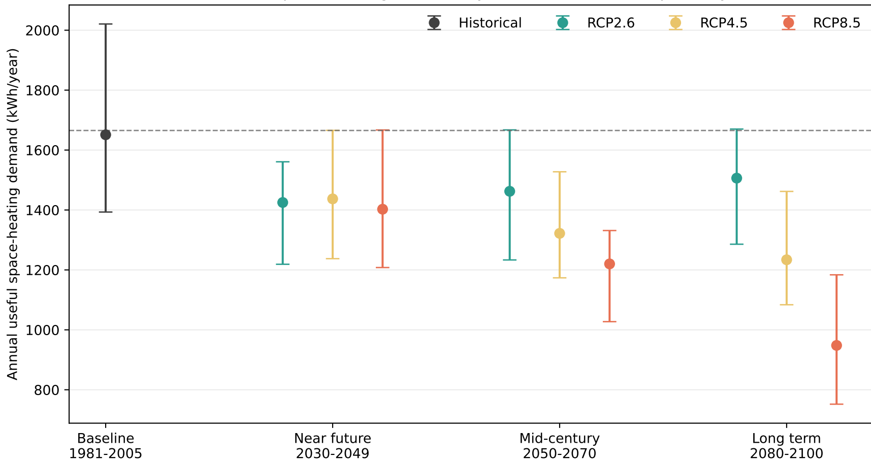
Annual space-heating demand by climate window and pathway
