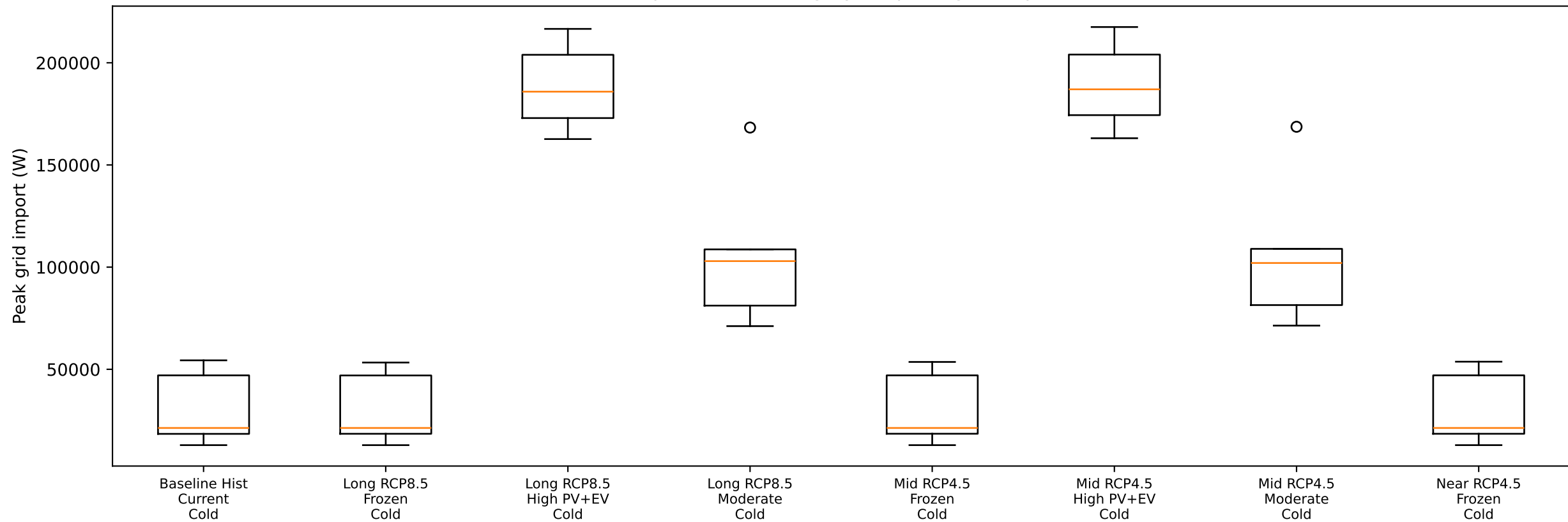
Output 3: cold-design-year peak grid import
