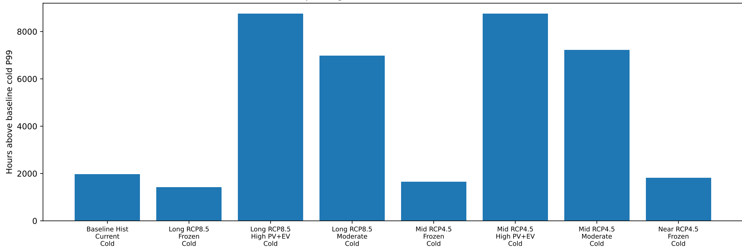
Output 3: grid-stress threshold exceedance
