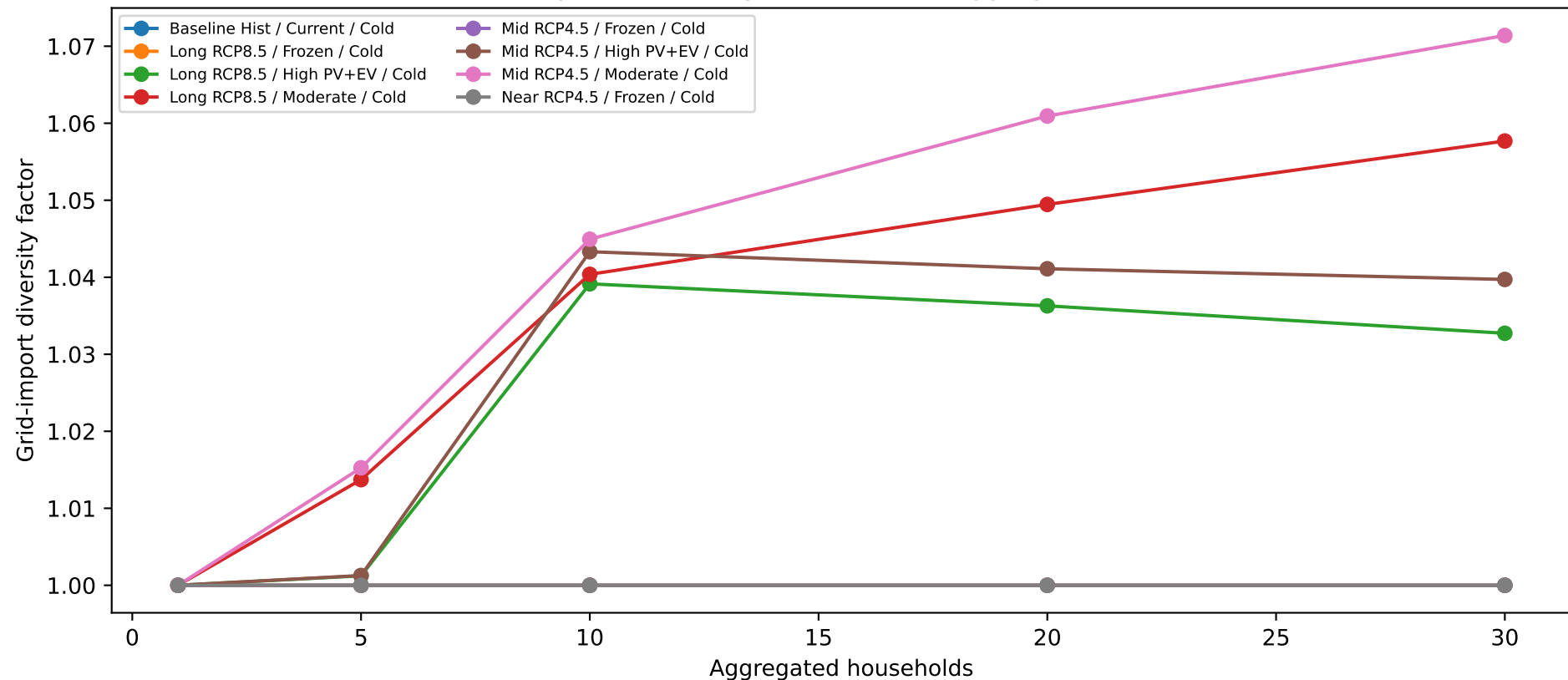
Output 4: diversity factor versus aggregation size
