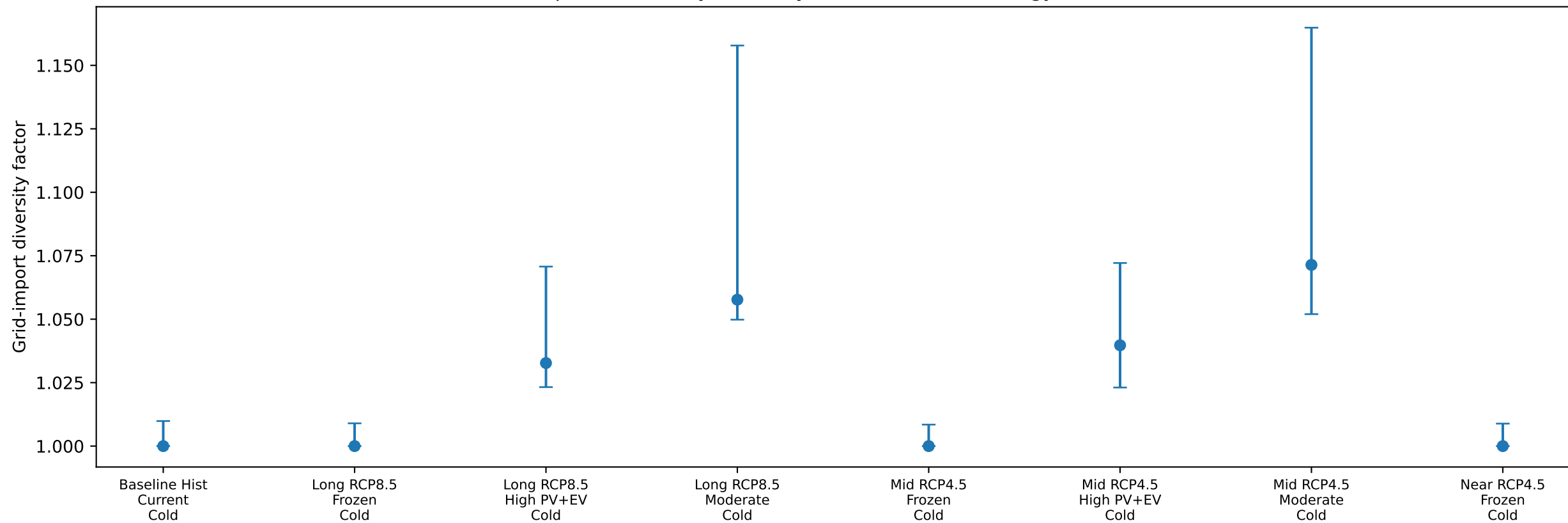
Output 4: diversity factor by climate and technology scenario
