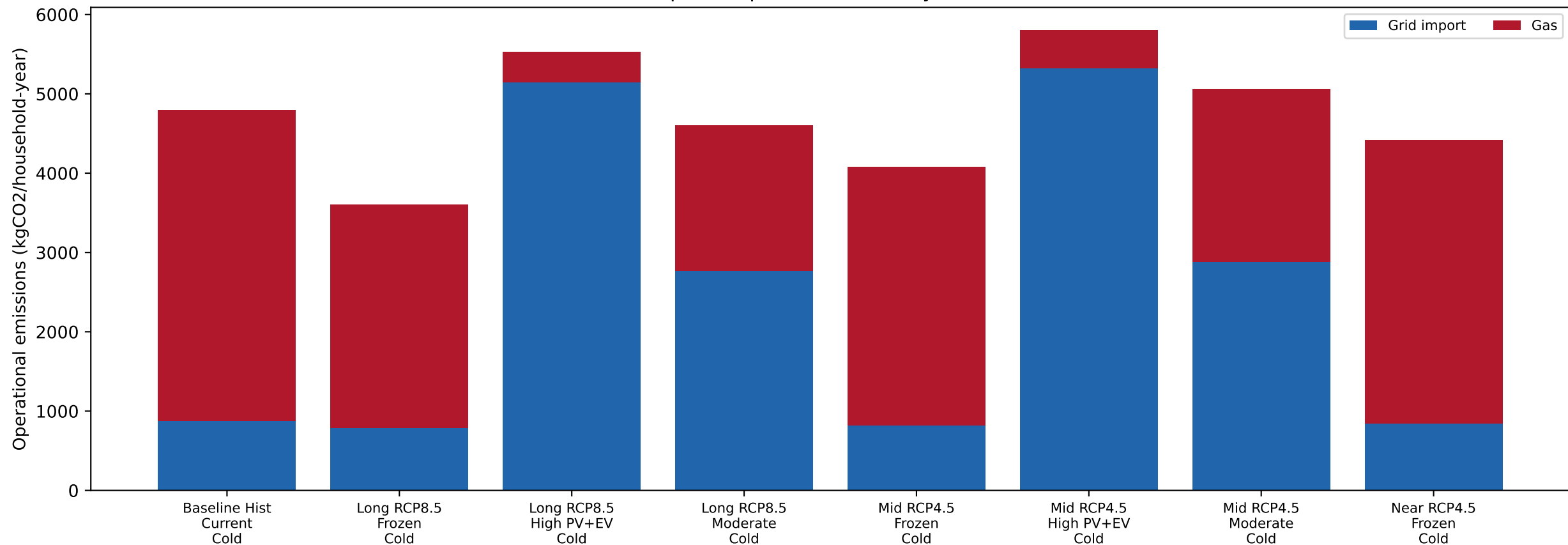
Output 5: operational CO2 by scenario
