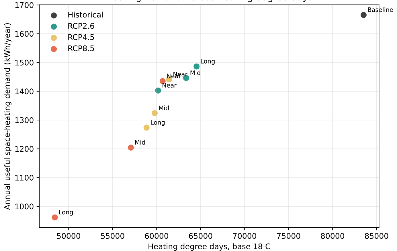
Heating demand versus heating degree days
