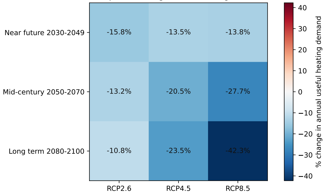
Annual space-heating demand change vs baseline
