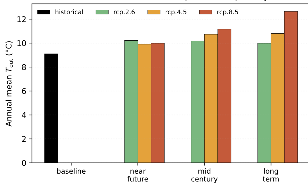
(c) Annual mean outdoor temperature, all pathways
