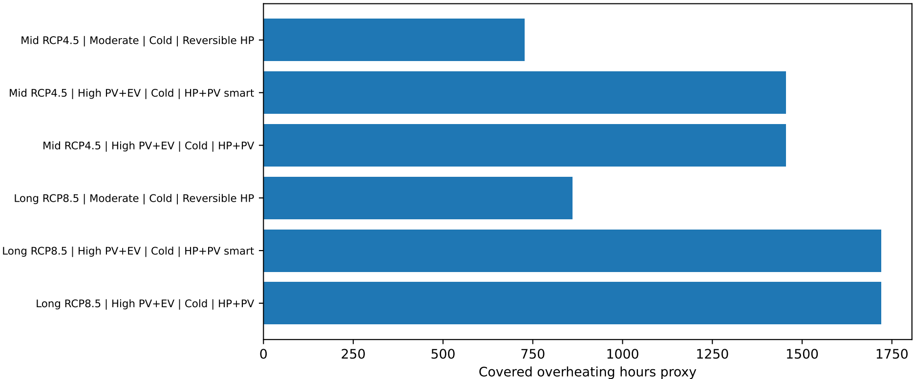
Output 6: reversible heat-pump adaptation proxy
