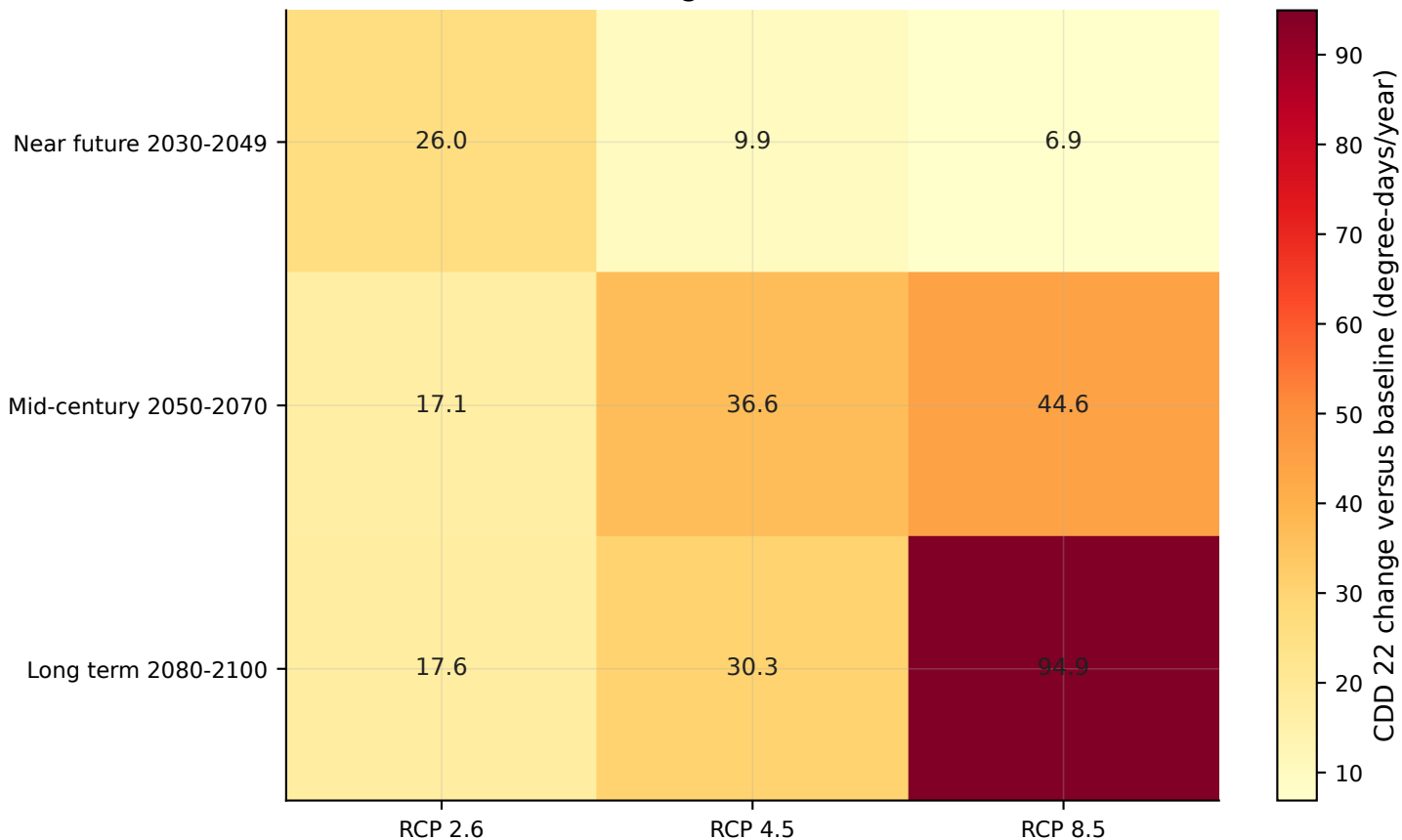
CDD absolute change versus historical baseline
