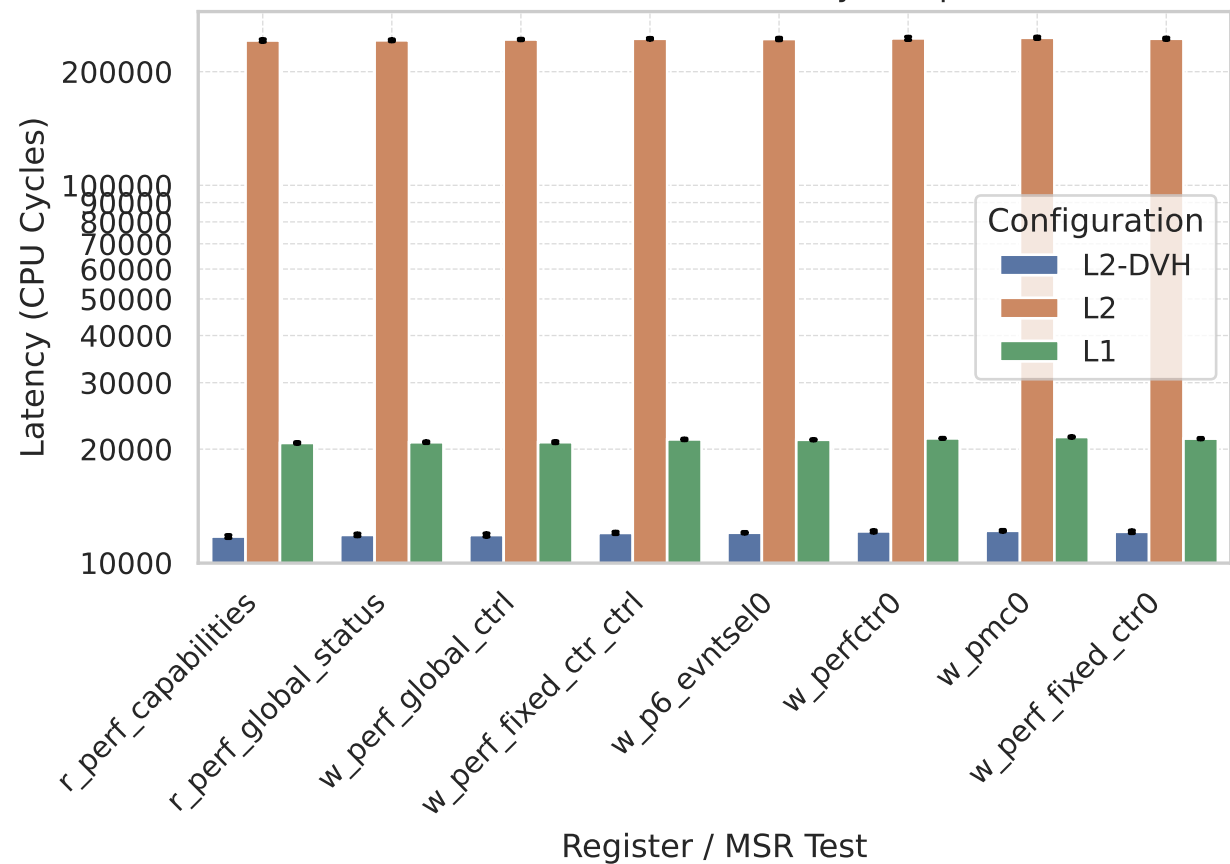
PMU Microbenchmark Latency Comparison
