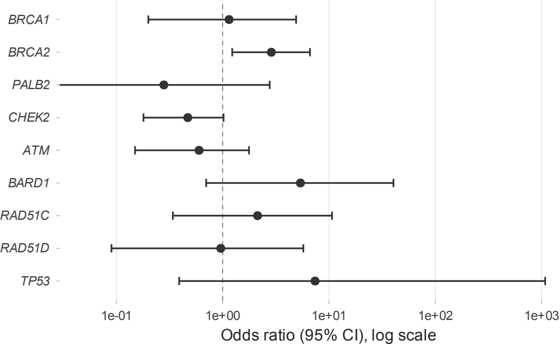
Figure A3. BBD, protein-truncating variants (n = 1,765)
