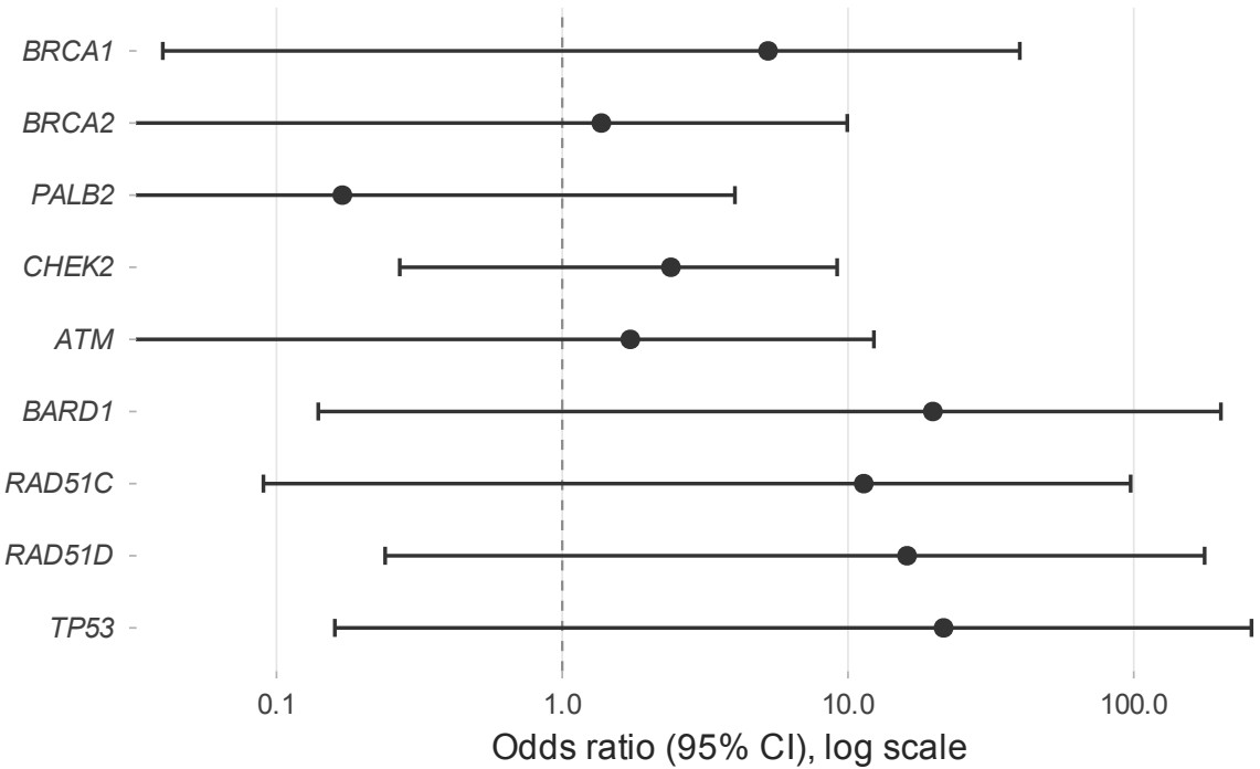
Figure A5. LCIS, protein-truncating variants (n = 139)
