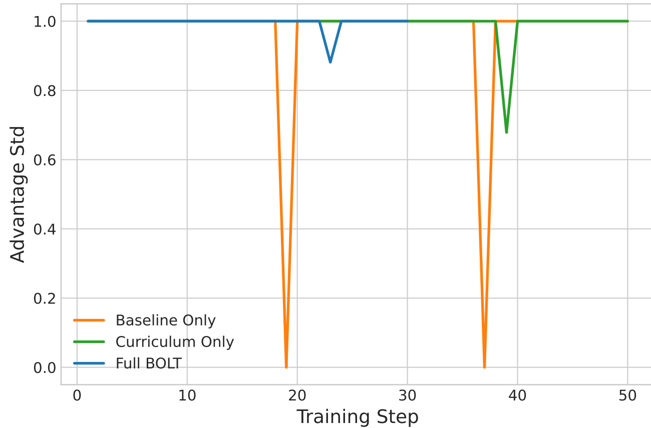
Advantage Standard Deviation
