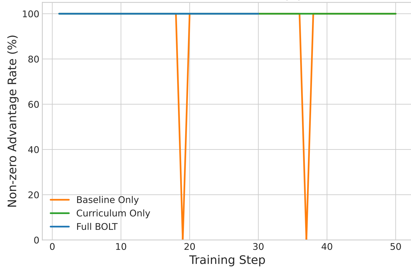
Rate of Non-zero Advantages ( |A| > 0.01 )
