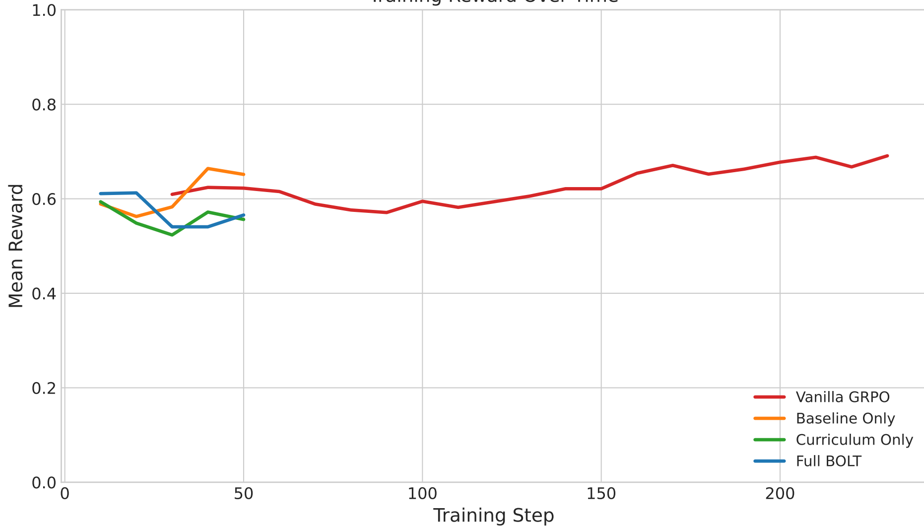
Training Reward Over Time
