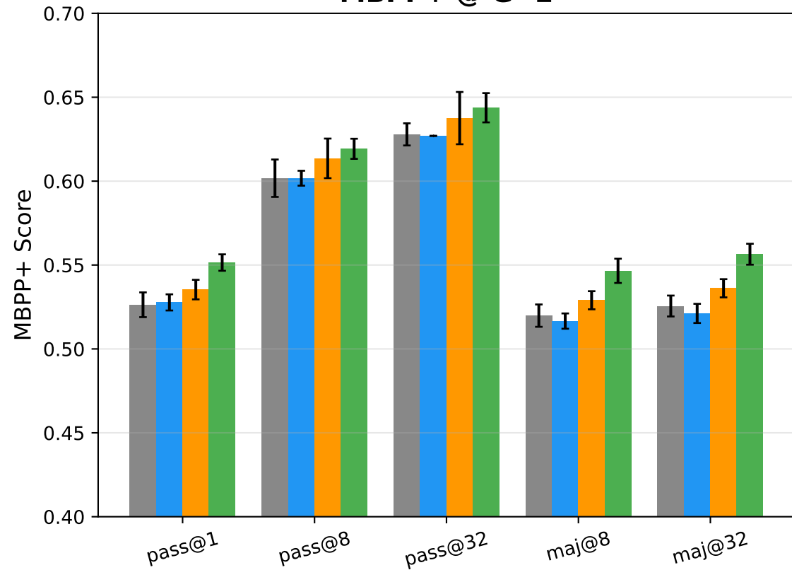
MBPP+ @ G=2
