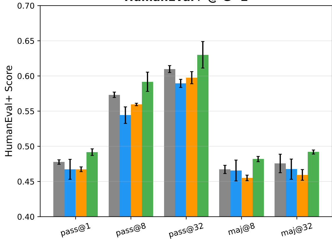
HumanEval+ @ G=2
