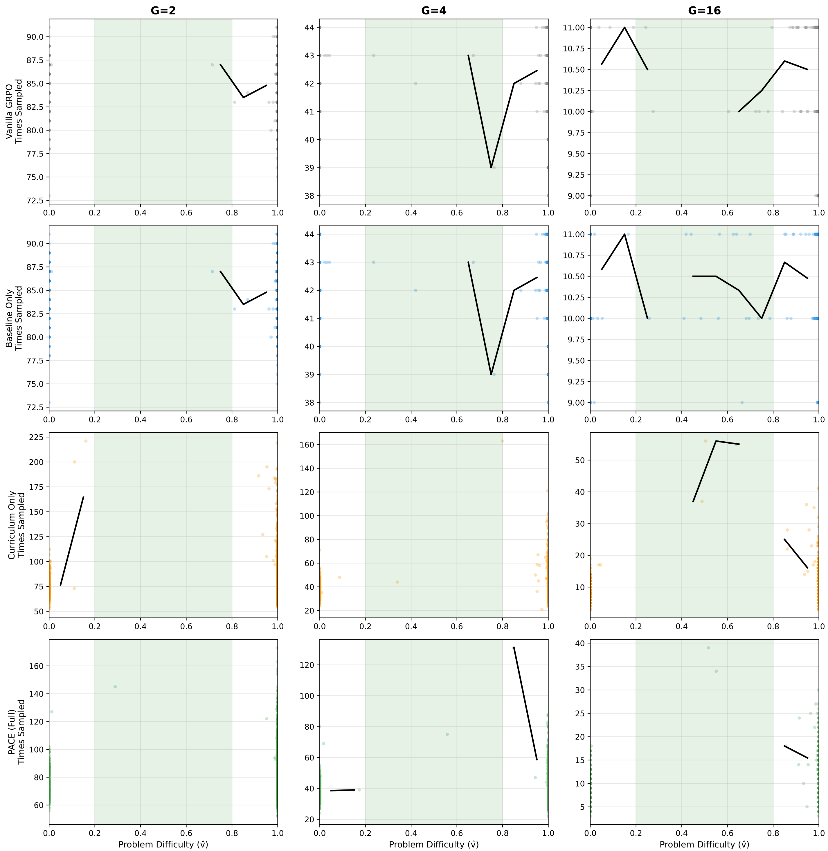
Revisit Count vs Problem Difficulty (Green = Learning Edge: 0.2 < \hat{v} < 0.8 )
