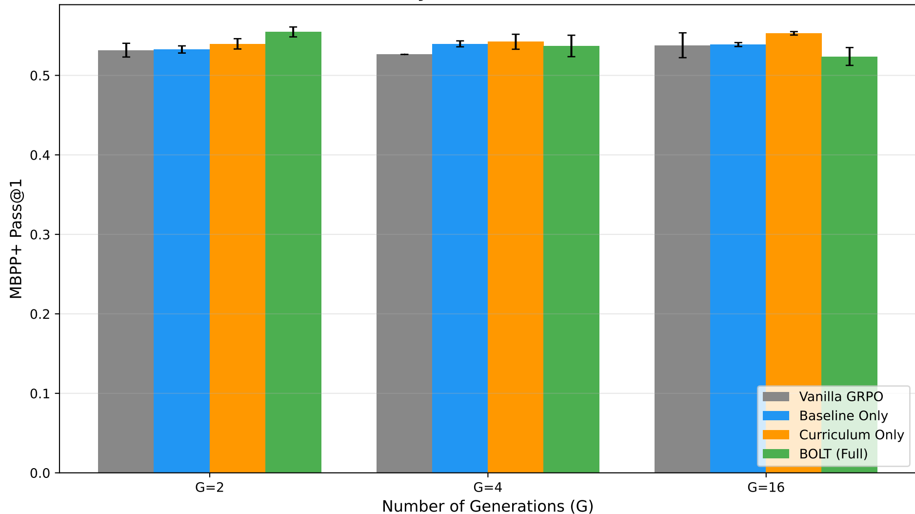
Final Performance by Condition and Generation Count
