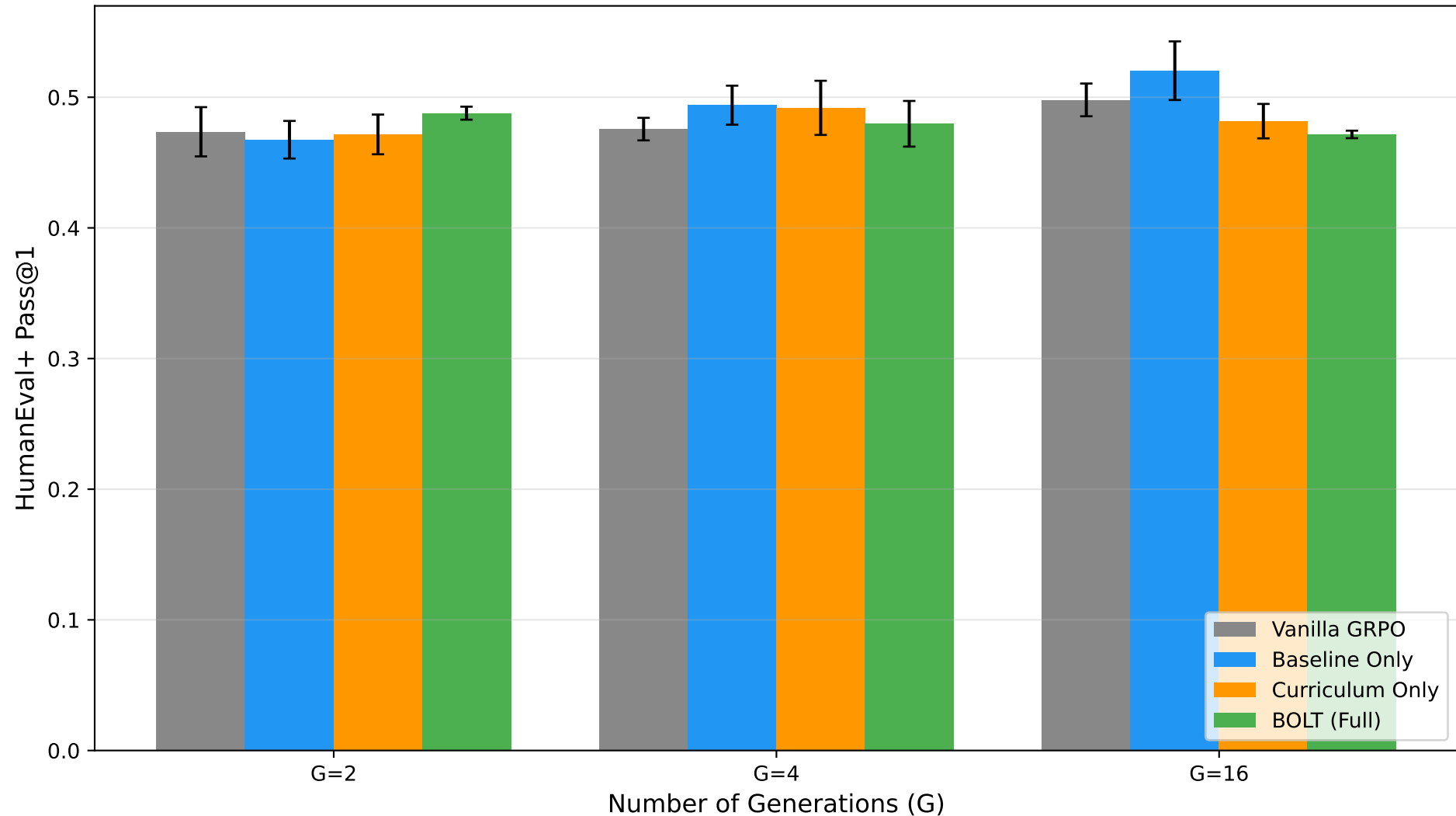
HumanEval+ Final Performance by Condition
