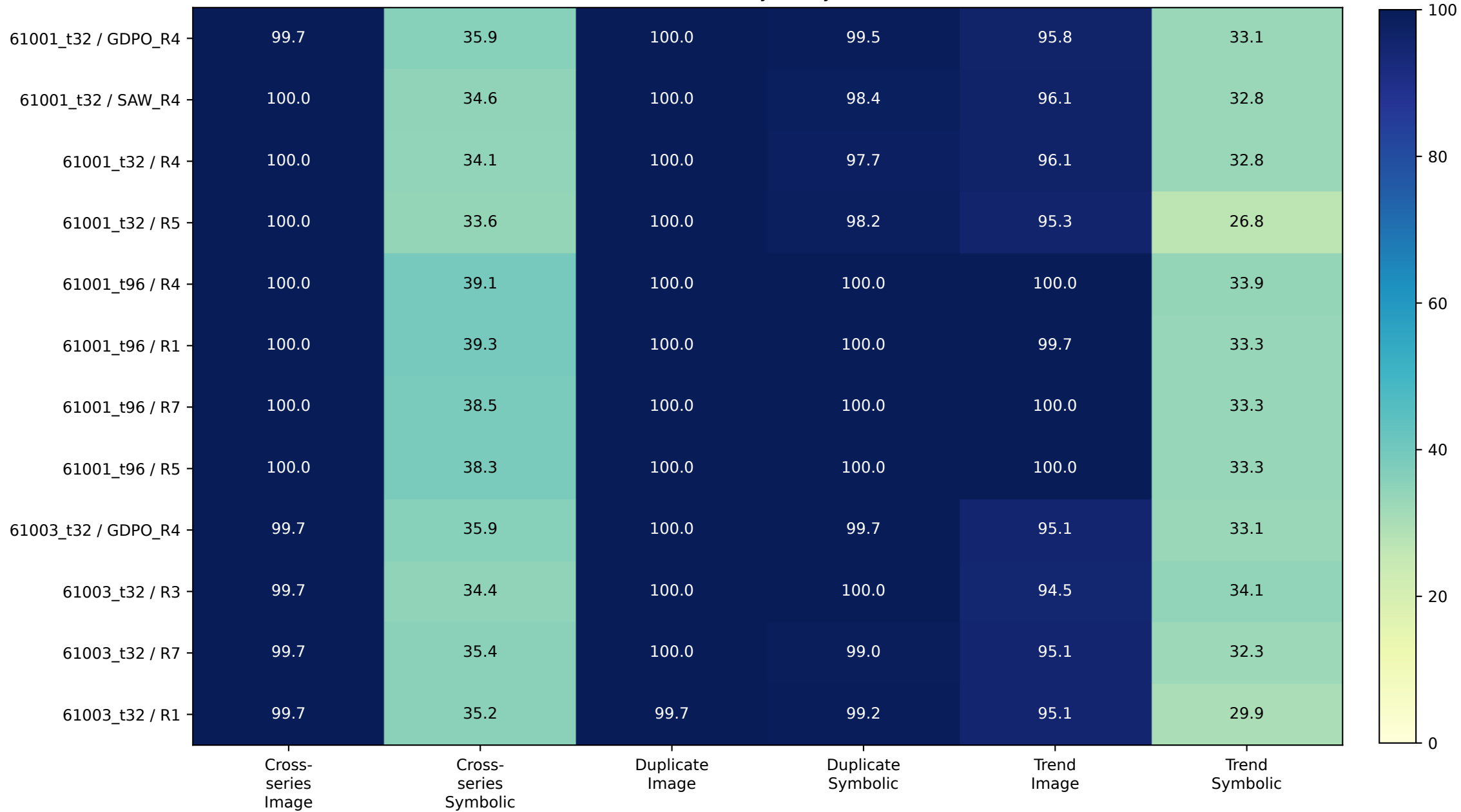
H32 exact correctness by family and interface (%)
