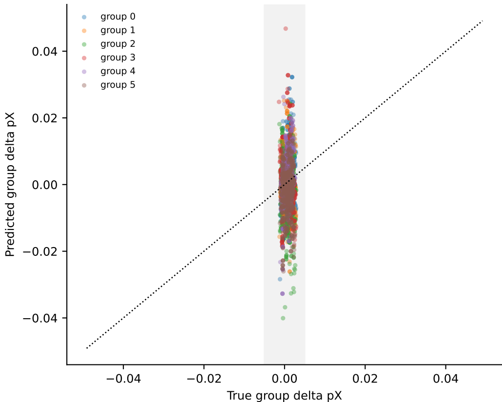
Frozen exact-selected r=1 ; n=64 , noise=0; 4320 group responses
