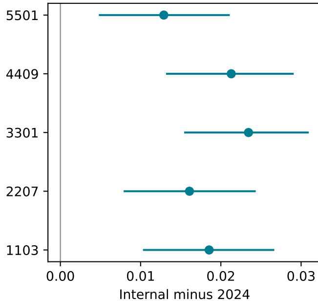
QWK gap
