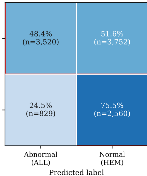
ConvNeXt V2 + FocusAugMix (Ours) Recall: ALL 48%, HEM 76%
