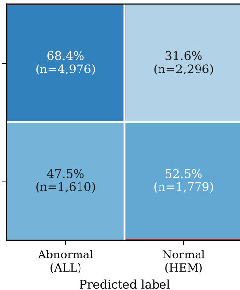
ConvNeXt V2, no_mix (baseline) Recall: ALL 68%, HEM 52%
