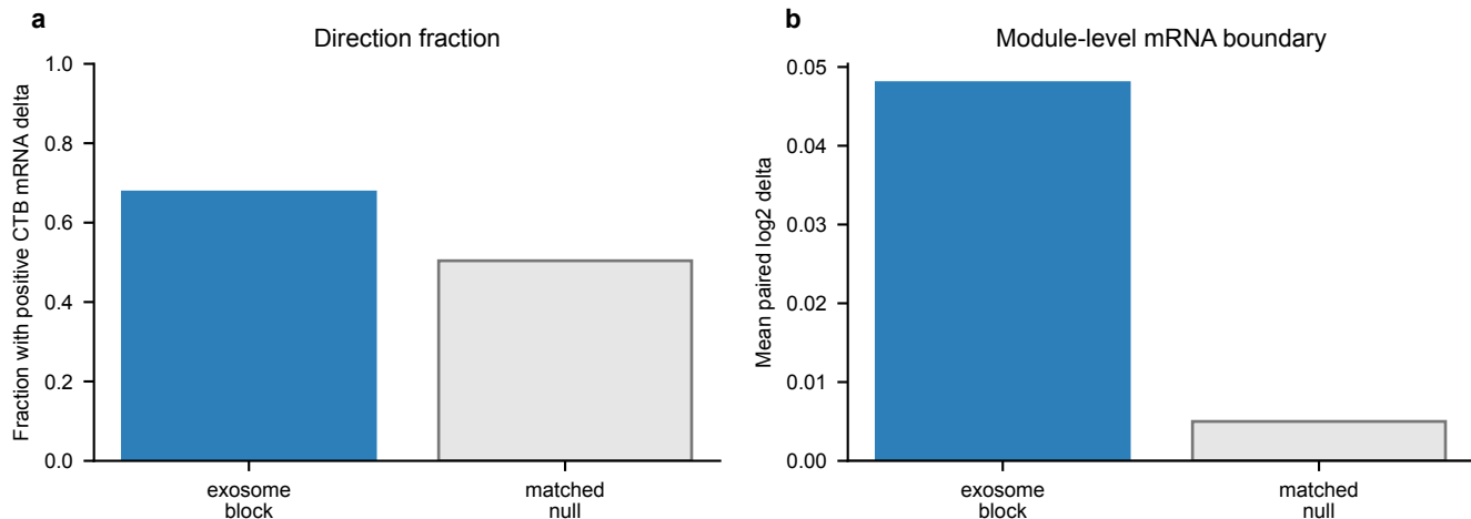
Figure 4. CTB mRNA boundary analysis and source-resolved model
