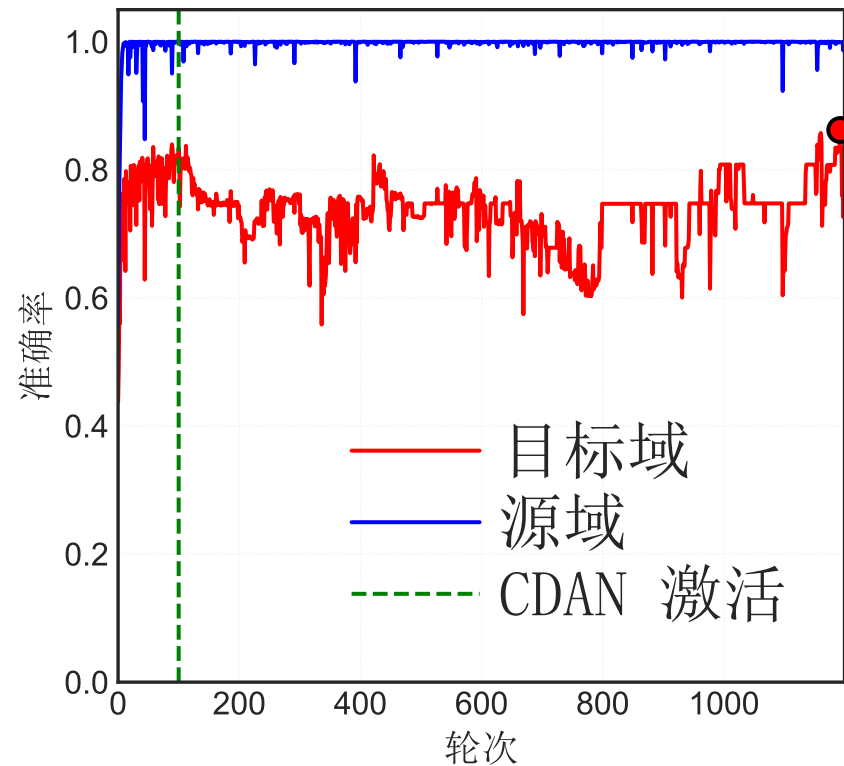
(a) 训练准确率
