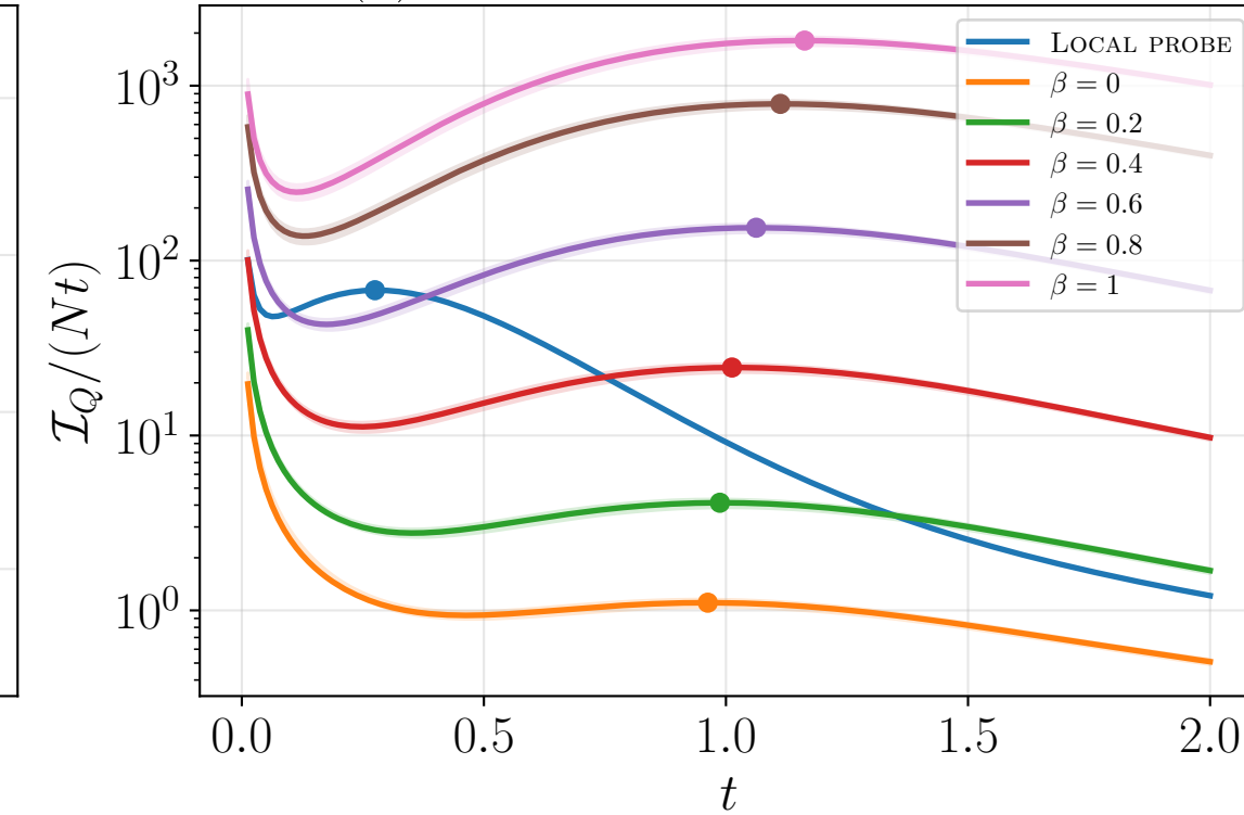
(b) Truncated : \alpha = 0.5, N = 80
