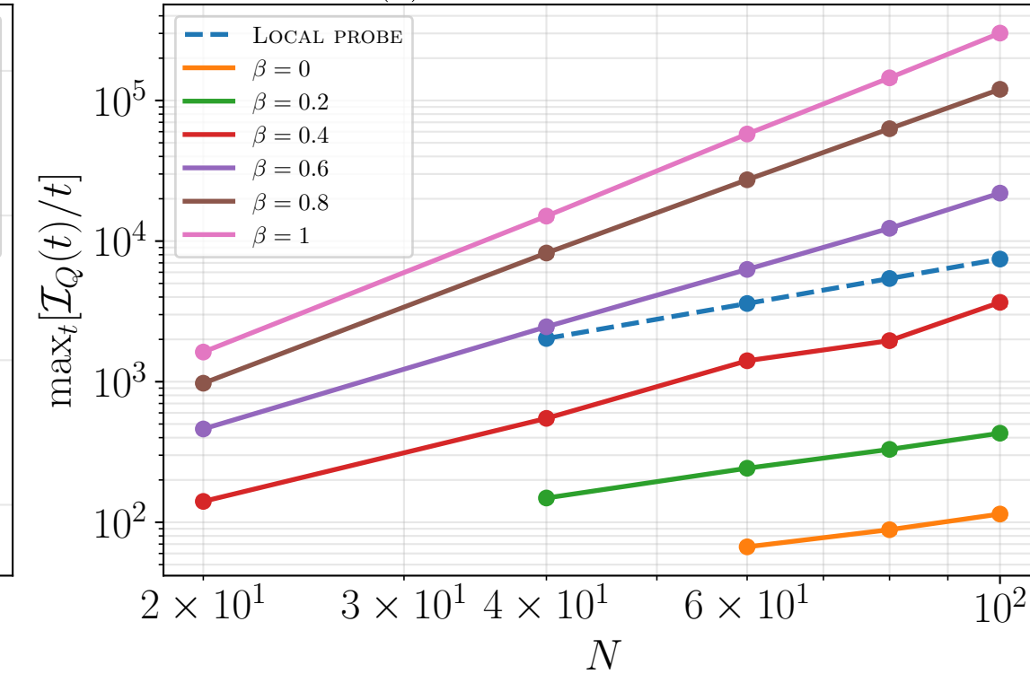
(c) Truncated : \alpha = 0.5
