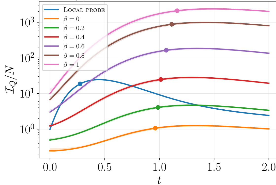
(a) Truncated : \alpha = 0.5, N = 80
