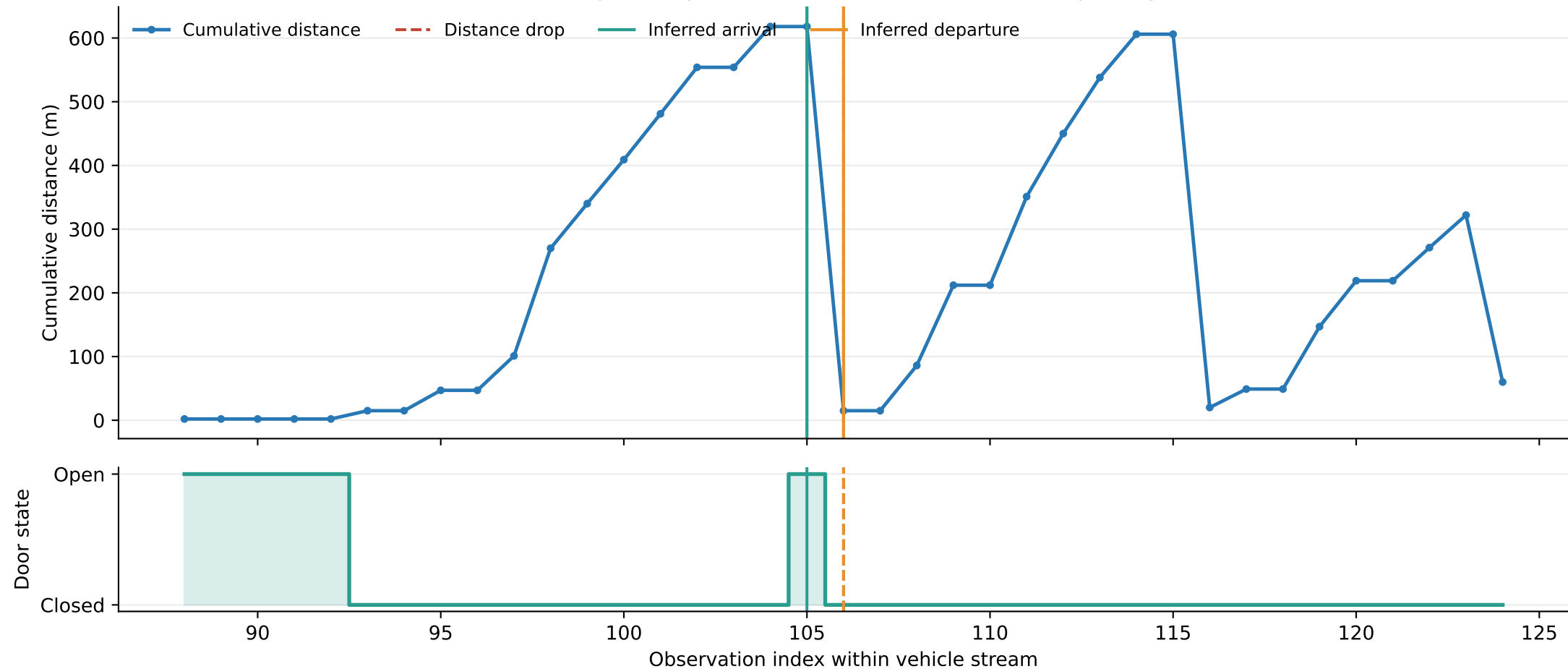
Dual-signal stop-event inference for one vehicle passage
