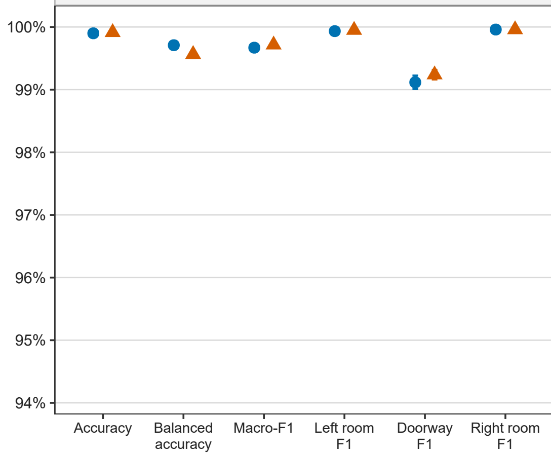
3-Partition
