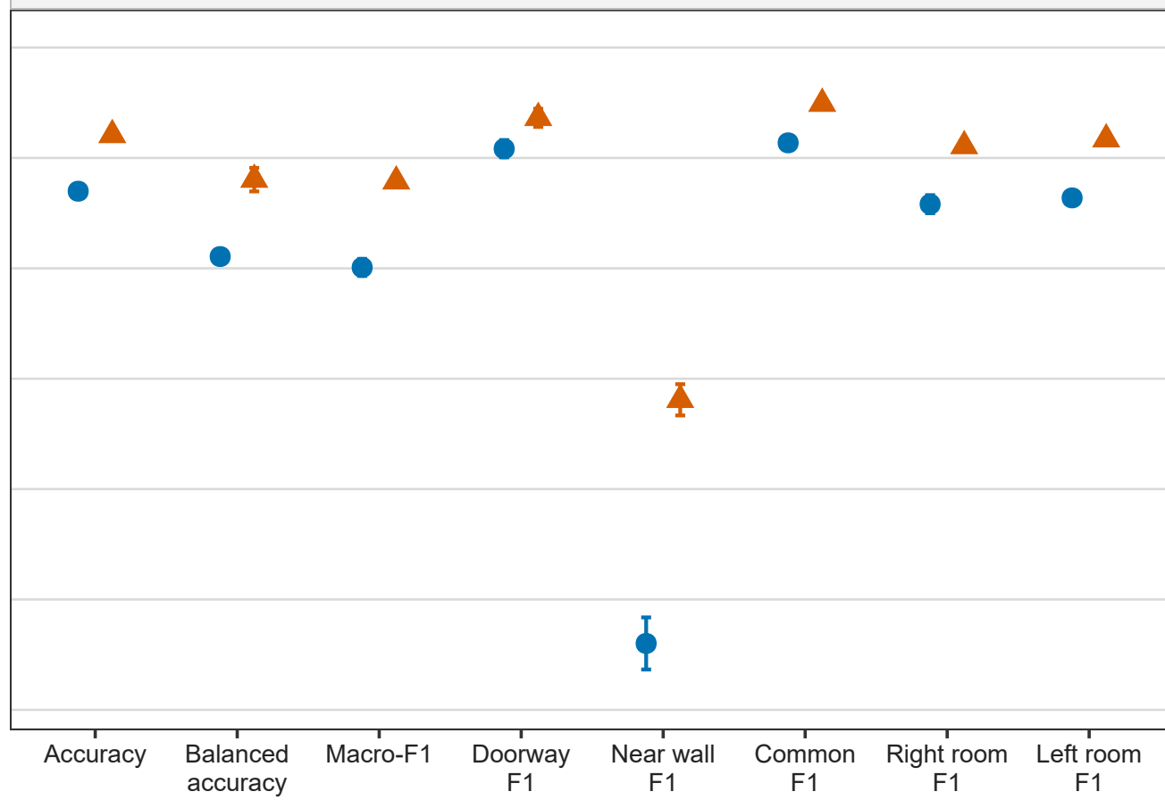
5-Partition
