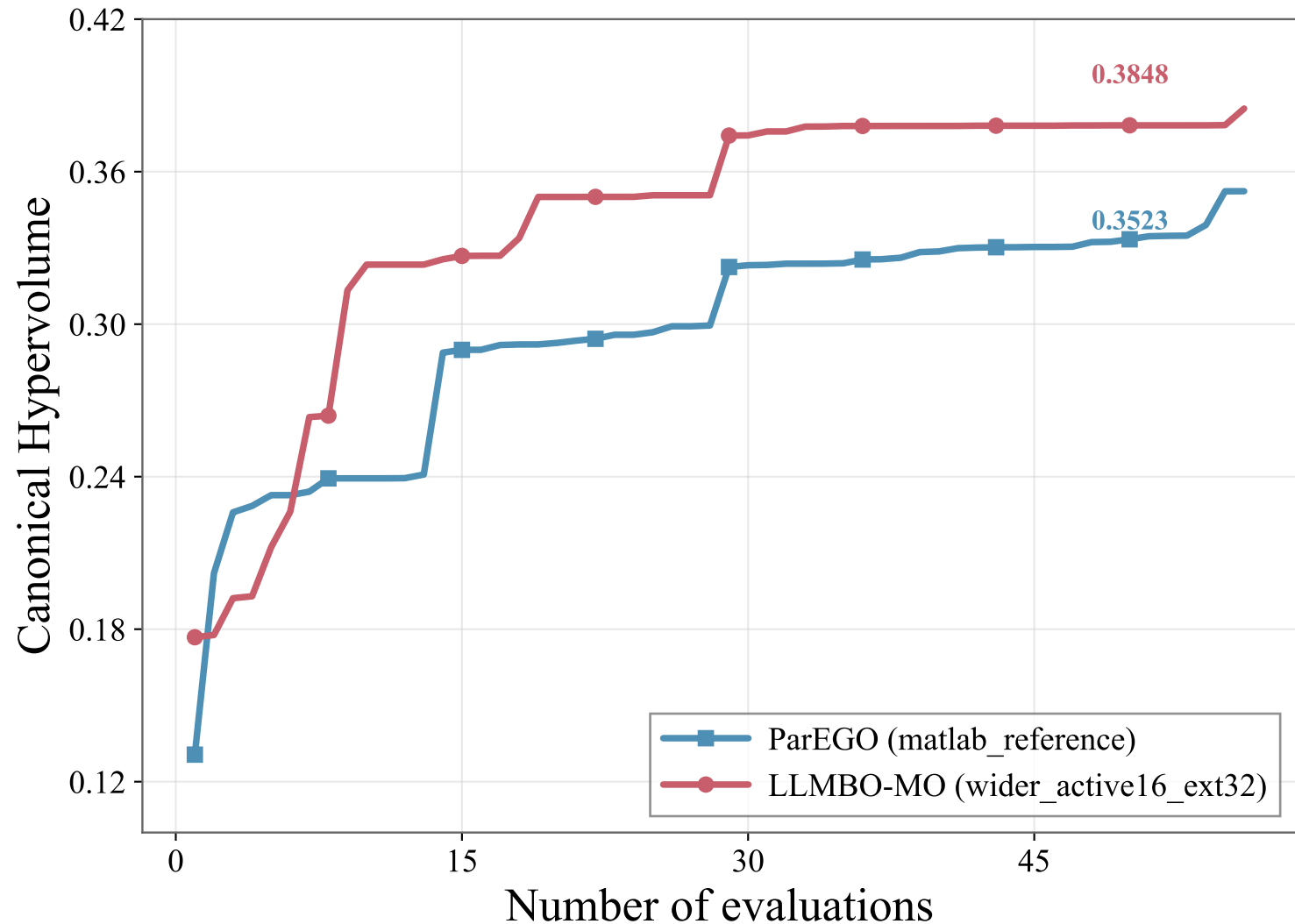
Seed 8409: LLMBO-MO vs ParEGO (50 iterations)
