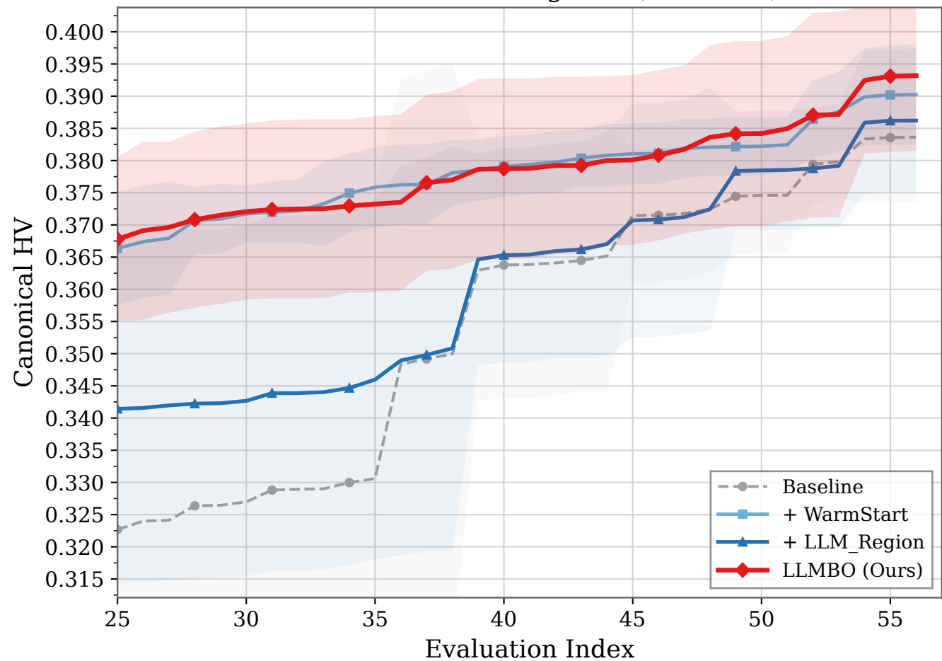
Ablation HV Convergence (Last 55%)
