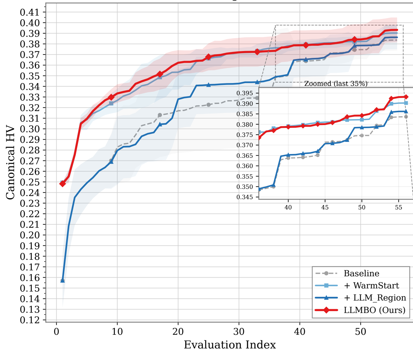
Ablation HV Convergence (Inset Zoom)
