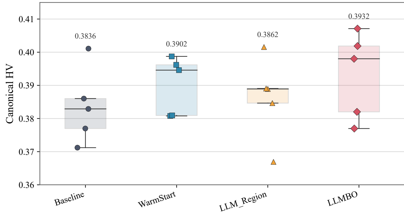
Ablation Canonical HV Distribution
