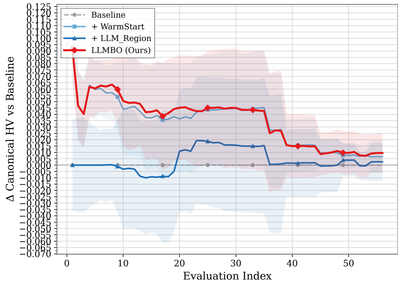
Ablation: HV Gain Over Baseline
