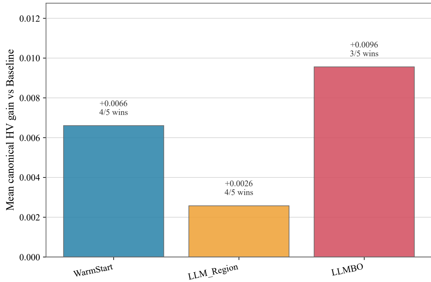
Ablation Gain Over Baseline
