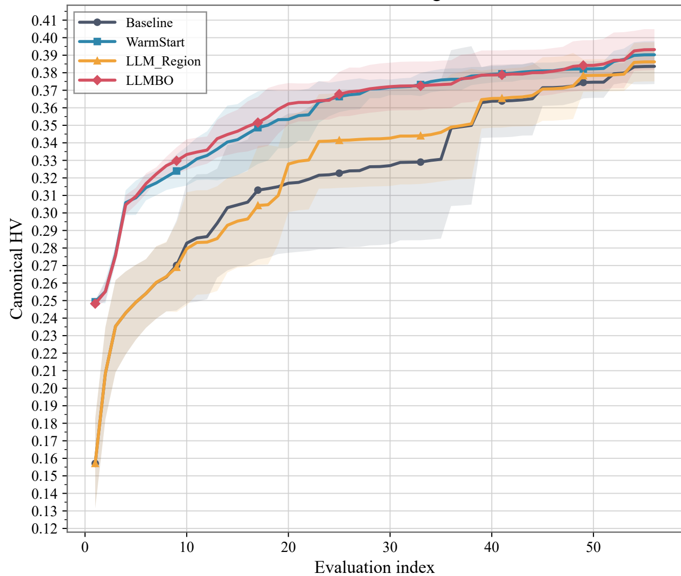
Ablation HV Convergence
