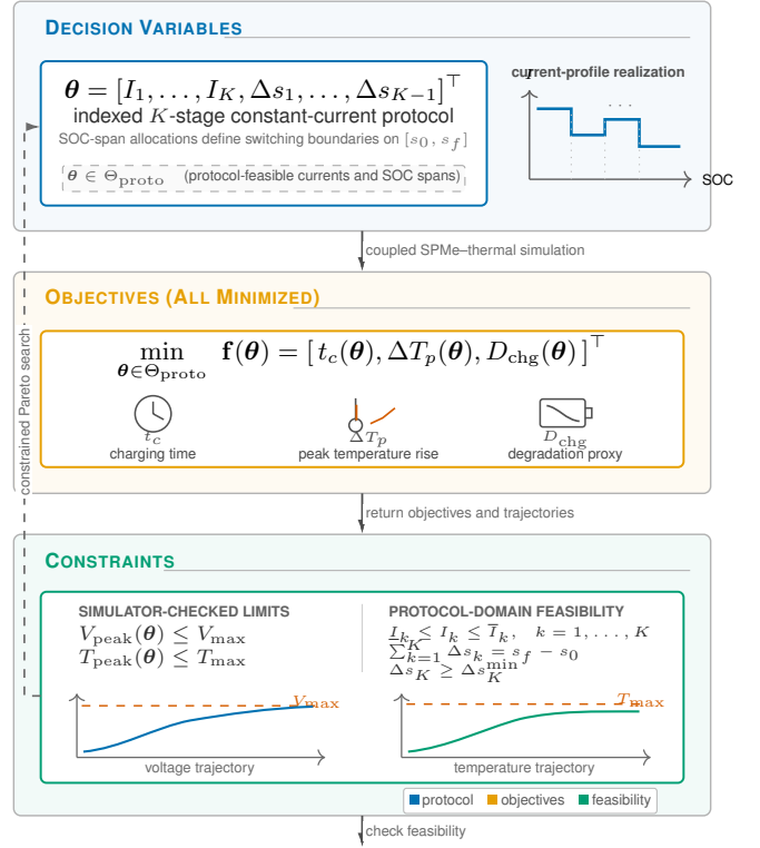
Fig. 1. Fast-charging design problem formulation. Protocol-feasible current and SOC-span coordinates are mapped through the coupled battery evaluator to three minimized objectives and simulator-checked operational limits; constrained Pareto search updates the protocol proposal.
