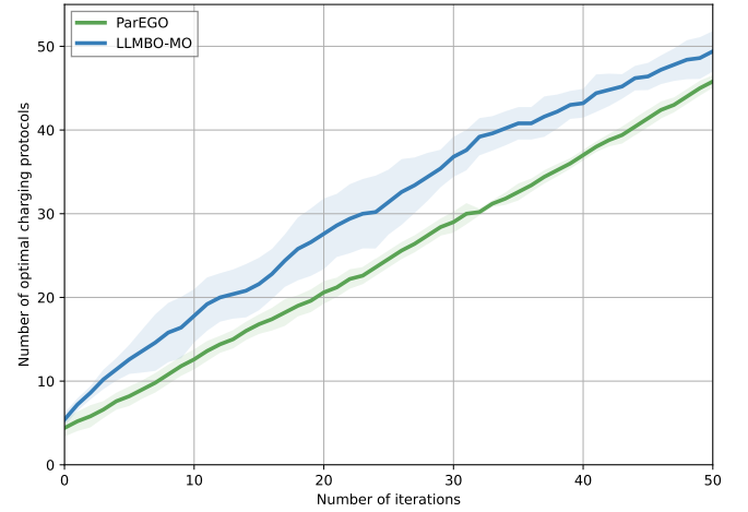
Fig. 5. Chen2020 Pareto-archive growth over 50 algorithmic iterations. Lines are five-run means and bands show across-run dispersion. An optimal charging protocol is a feasible Pareto-nondominated archive entry.
