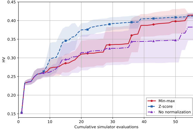
Fig. 6. Chen2020 objective-preprocessing sensitivity over five archived seeds. Lines show mean HV and bands show one sample standard deviation.
