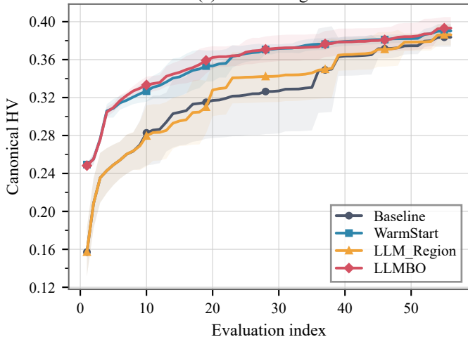
(a) HV convergence
