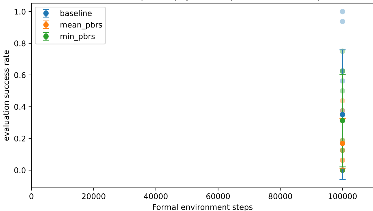
evaluation_success_rate at preregistered 100,000-step endpoint (intermediate eval episode payloads unpublished; no interpolation)
