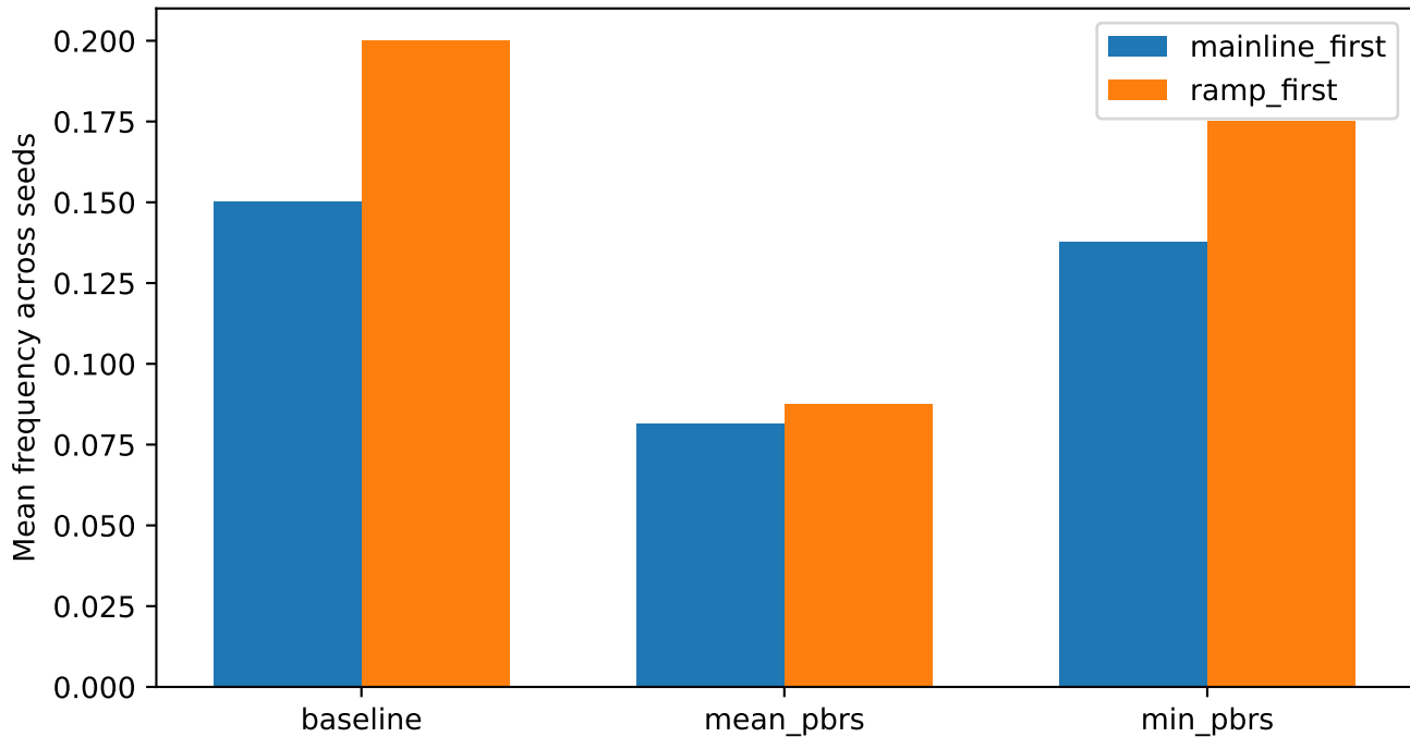
Convention frequencies at step 100000
