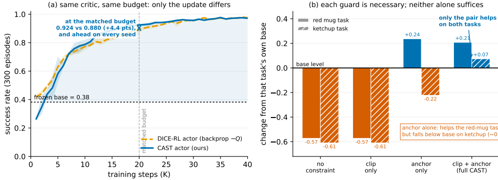
Figure 4: Why CAST wins, and why it needs both guards. (a) robomimic square, 300-episode evaluations; line is the seed mean, band the min-max over three seeds. Both arms share the base, critic, data, replay and budget — only the actor update differs. At the matched 20K budget CAST reaches 0.924 against the backpropagated actor’s 0.880, and is ahead on every seed; both converge near 40K, so the gain is in what the update extracts per step, not in the asymptote. (b) the constraint factorial, plotted as change from each task’s own base so that zero is “did nothing”. Removing the anchor is fatal whether or not the step clip is present (−0.57 and −0.61: both arms collapse to 0.000 success), which is the paper’s central negative result — many individually capped steps still compound into a walk off the data. The anchor alone survives but is not reliable: +0.24 on the red-mug task, −0.22 on ketchup, i.e. worse than not fine-tuning at all. Only the pair is positive on both. Neither guard is sufficient; the claim is about the pair.
