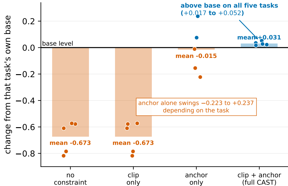
(b) only the full pair clears base on every task (5 tasks)
