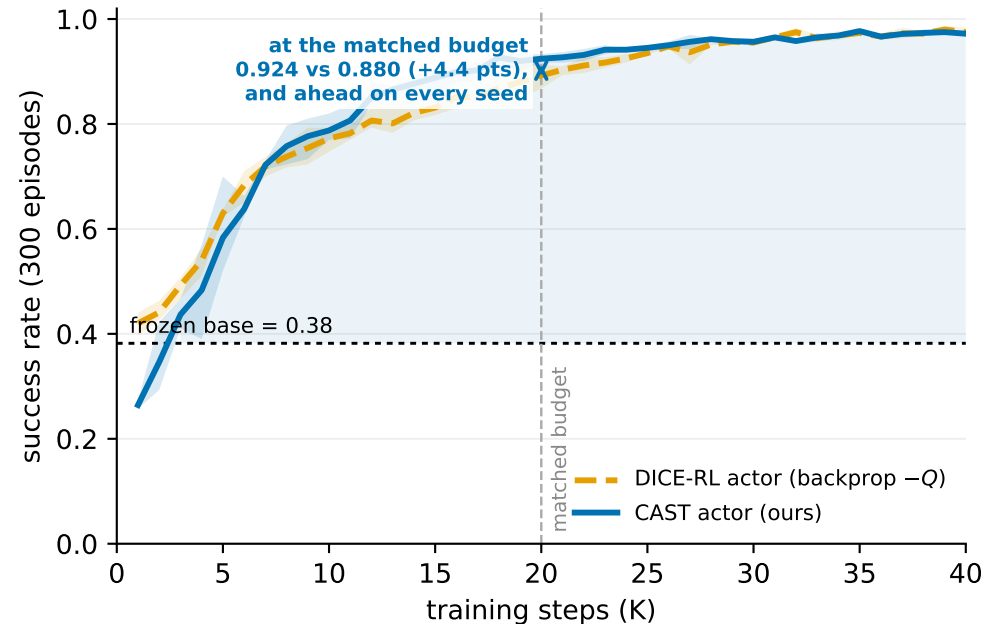
(a) same critic, same budget: only the update differs
