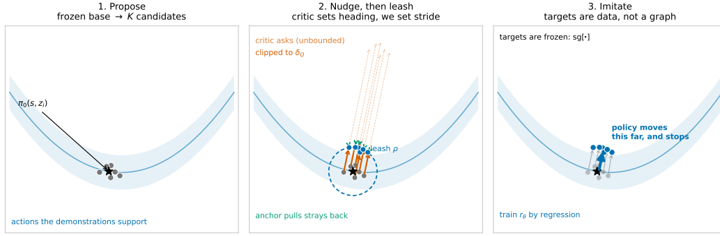
Figure 3: CAST in three steps (schematic). Left : the frozen base maps noise to K candidate actions, which lie on the thin band of actions the demonstrations support. Middle : the critic’s gradient points off that band (faint arrows, unbounded); CAST keeps only its direction and takes a step of length at most \delta_Q (solid), then the dead-zone anchor pulls back any candidate that has left the leash of radius \rho (green). Right : the displaced targets are detached and the residual head is regressed onto them, so the policy moves a bounded distance and stops. The base is any frozen noise-to-action map.
