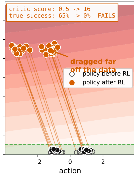
(b) backpropagating the critic
