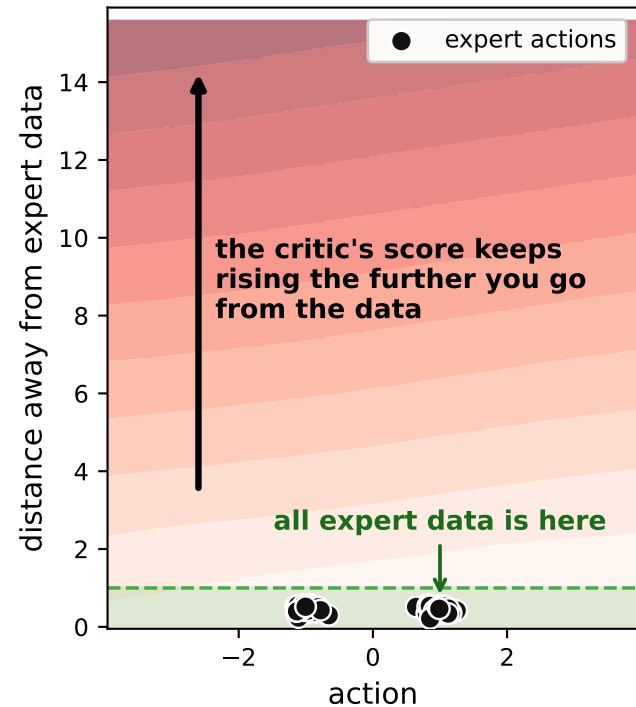
(a) what the critic believes
