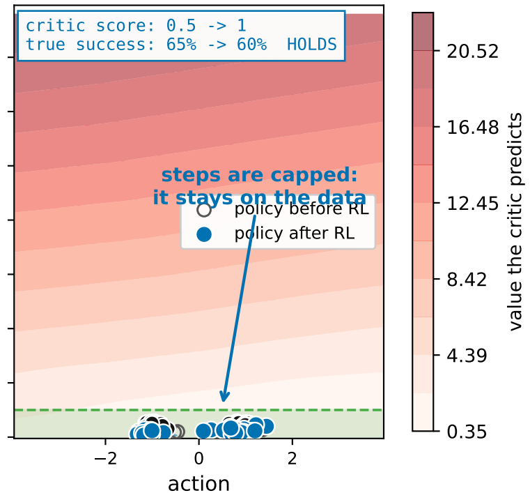
(c) our bounded field update
