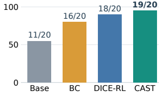
Autonomous success (%)
