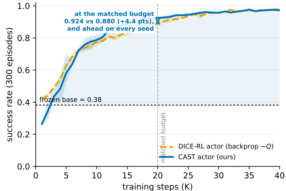
(a) same critic, same budget: only the update differs
